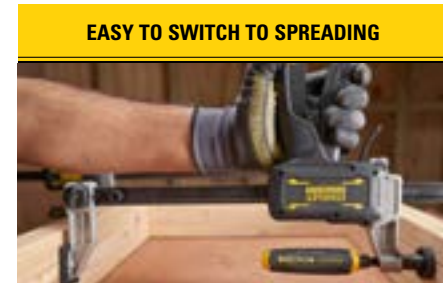
EASY TO SWITCH TO SPREADING Quick-change mechanism without additional tools to switch from clamping to spreading.
